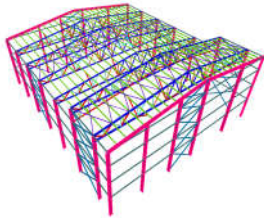
CRUSHING STRUCTURE (MALATYA)
